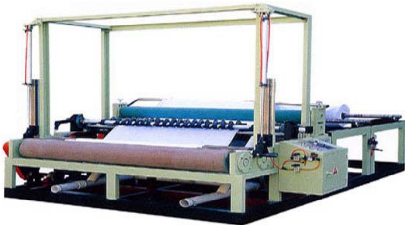
YX-FFJ-1092/1575 Cutting And Rewinding Machine
