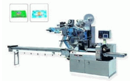
YX-10 wet tissue packing machine
